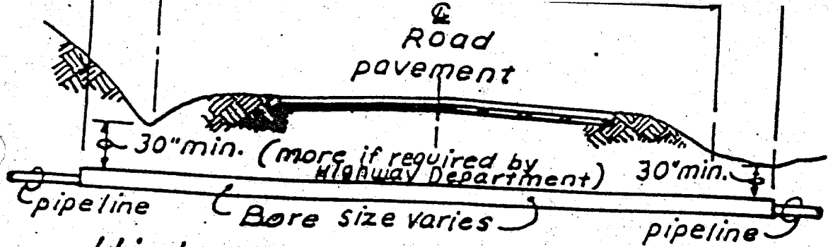
Highway-Street-Driveway Bore No Scale
